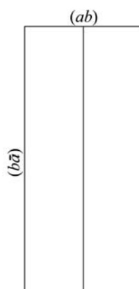
Fig. 1.2.6.18. The two settings for frieze groups. For the second setting, printed vertically, the page must be turned 90° clockwise or viewed from the right-hand side.
