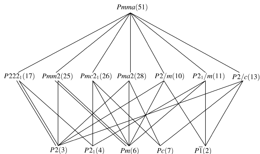
Fig. 2.4.4.1. Graph of the translationengleiche subgroups of the space group Pmma .
