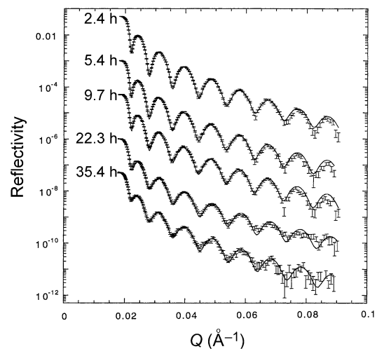
Fig. 2.9.7.1. Measured neutron reflectivities from boron bilayers [from Smith et al. (1992)].
