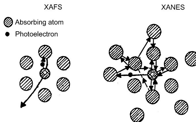
Fig. 4.2.3.5. Schematic representations of the scattering processes undergone by the ejected photoelectron in the single-scattering (XAFS) case and the full multiple-scattering regime (XANES).
