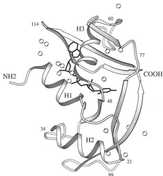
Fig. 23.4.4.11. Overall structure of RNase A. The overall structure of the d(CpA) complex of RNase A is shown as a ribbon drawing using MOLSCRIPT (Kraulis, 1991). The conserved water molecules are shown as white spheres and the d(CpA) inhibitor in black. The three helices are labelled H1, H2 and H3. Reprinted with the permission of Cambridge University Press from Zegers et al. (1994). Copyright (1994) The Protein Society.
